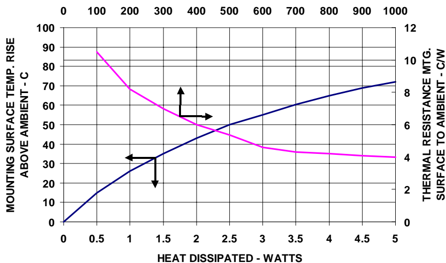
THermal PERFORMANCE - TS-54030-AD AIR VELOCITY - FT. PER MINUTE
