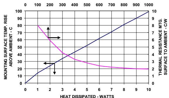
THERMAL PERFORMANCE - TS-54045-AD - 1.5” AIR VELOCITY - FT. PER MINUTE
