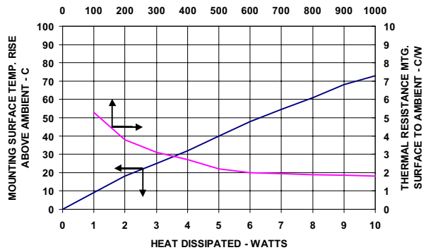
THERMAL PERFORMANCE - TS-54045-AD - 2.5” AIR VELOCITY - FT. PER MINUTE
