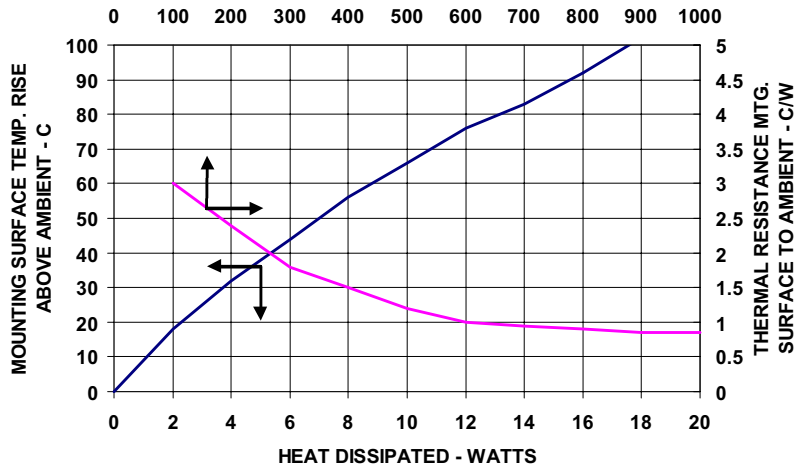
THERMAL PERFORMANCE - TS-54046-AD AIR VELOCITY - FT. PER MINUTE
