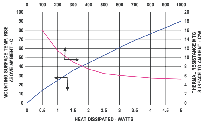
THERMAL PERFORMANCE - TS-54060-AD / ADVT AIR VELOCITY - FT. PER MINUTE
